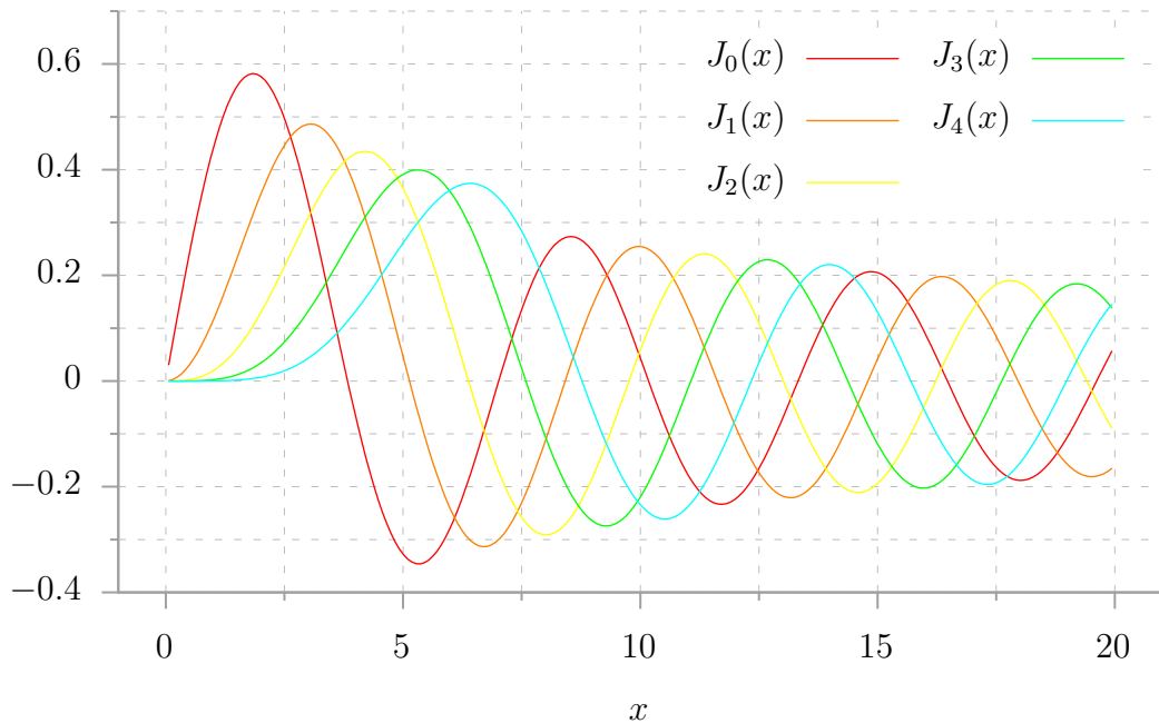
First Kind Bessel functions
